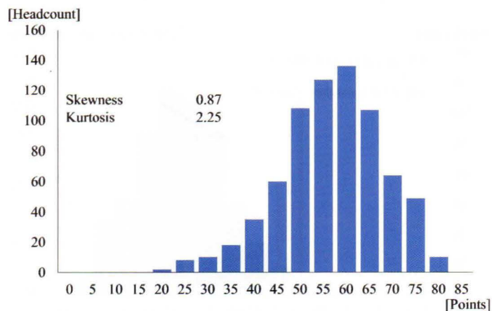
Fig. 2. Distribution of the physical fitness results The results were p-value = 0.0776, skewness = 0.8660, and kurtosis = 2.2460, showing a normal distribution.
